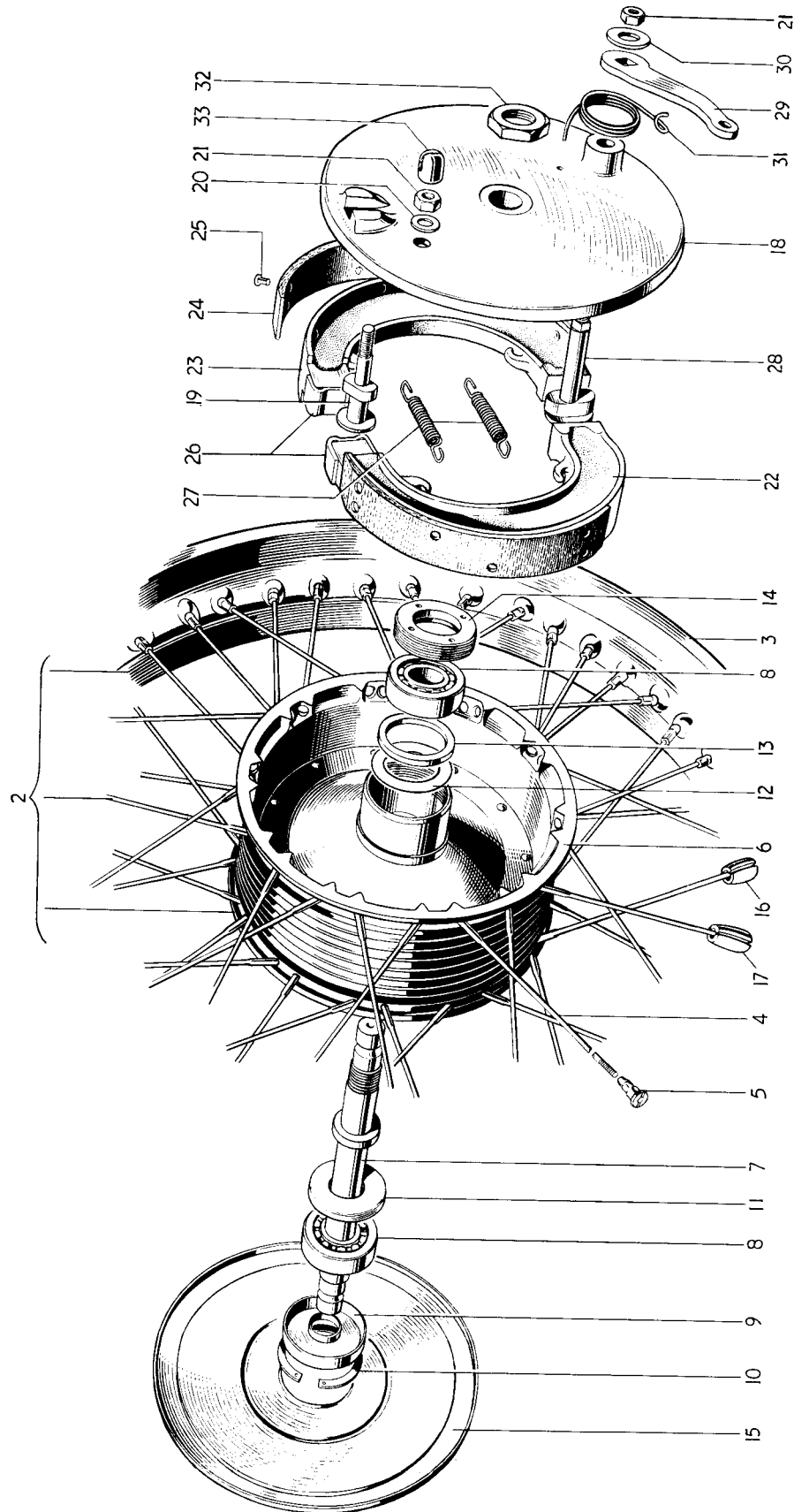
Fig. 19. FRONT WHEEL
