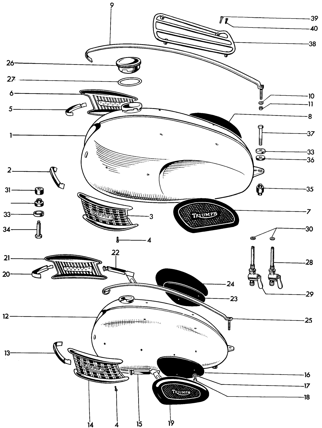
Fig. 22. PETROL TANKS
