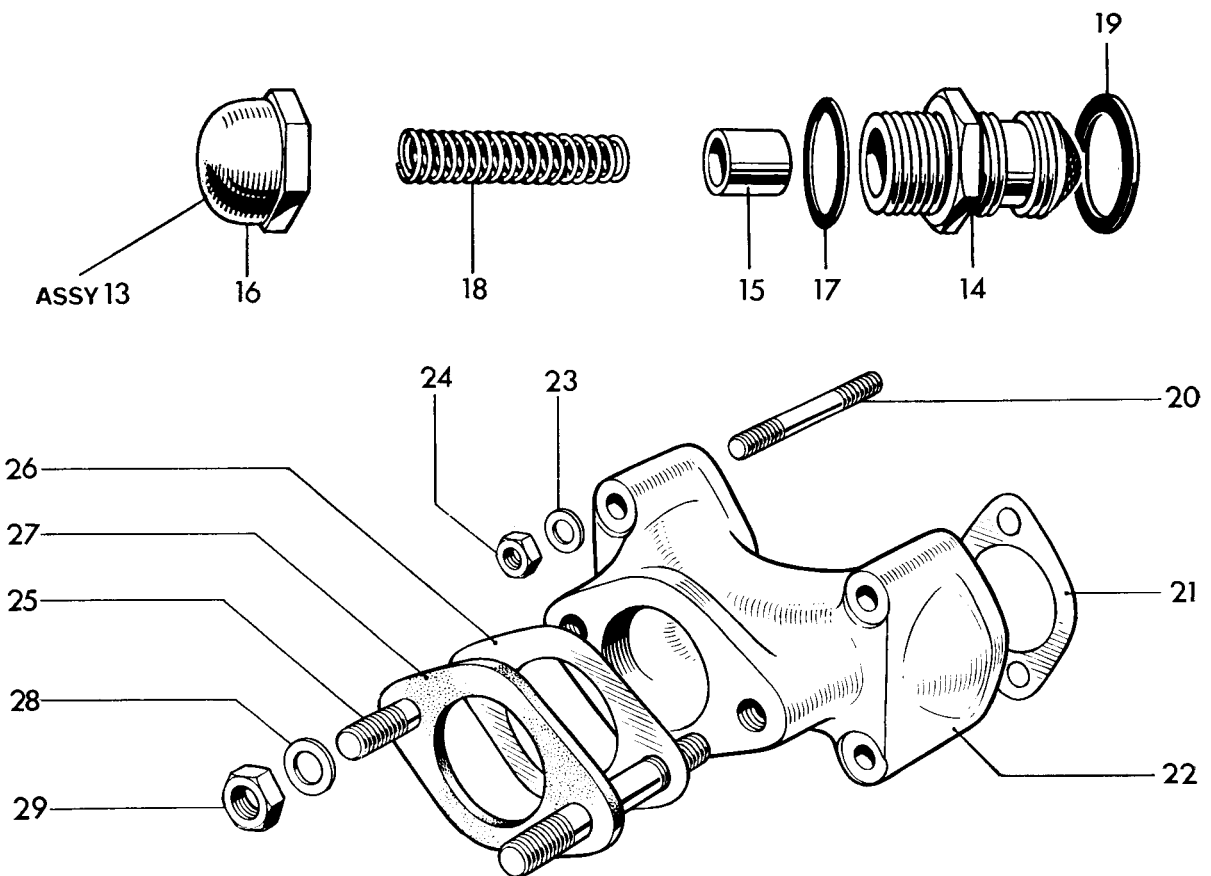
Fig. 3. OIL PUMP AND RELEASE VALVE AND MANIFOLD
