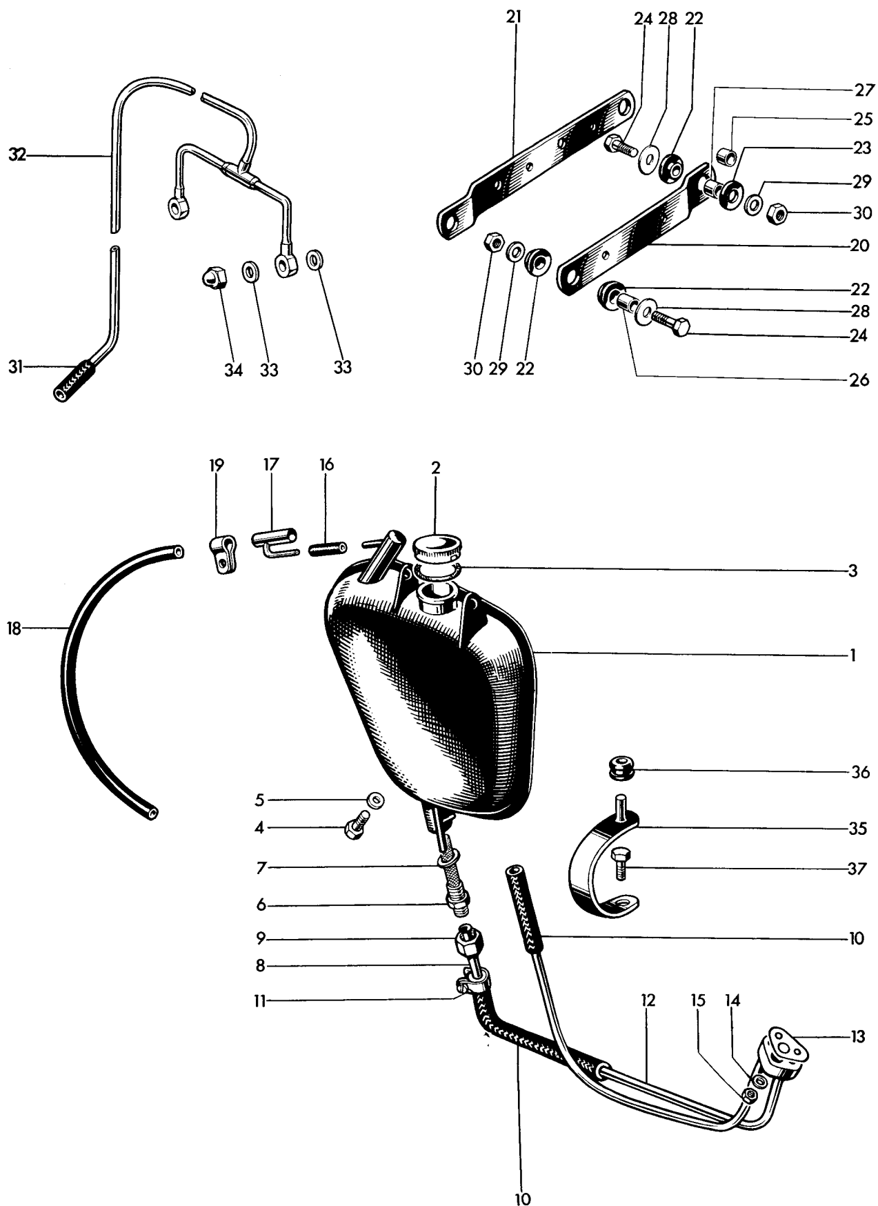
Fig. 23. OIL TANK
