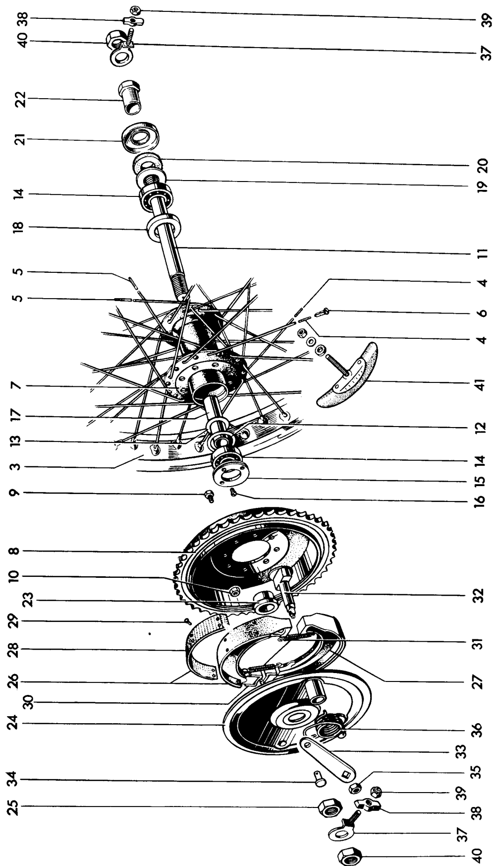
Fig. 20. REAR WHEEL
