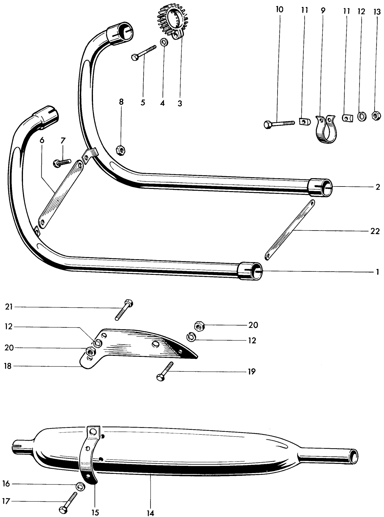
Fig. 15. EXHAUST PIPES AND SILENCERS
